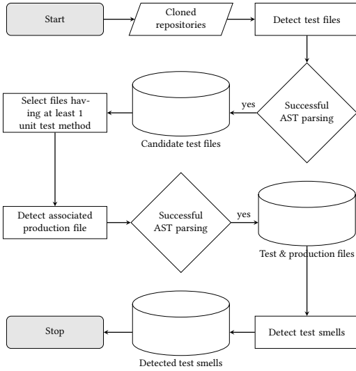
Figure 1: Overview of the Detection Phase process.
