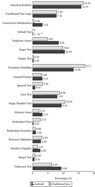
Figure 2: The distribution of the different test smell types in traditional Java and Android applications
