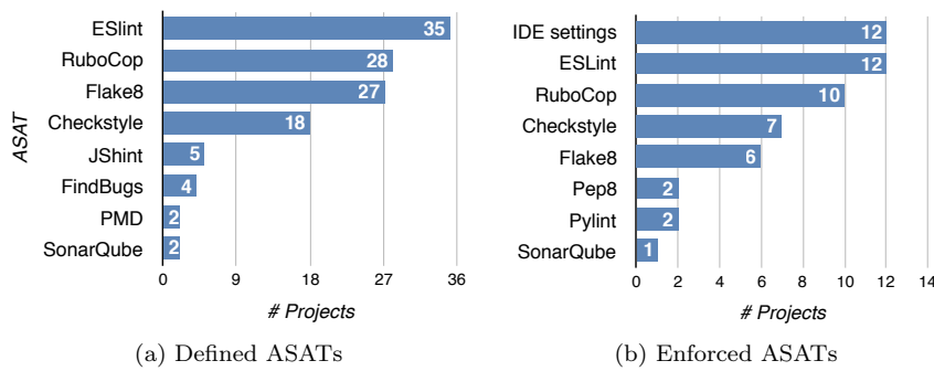
Fig. 8: The Most Relevant ASATs in the Analyzed Open-source Projects
